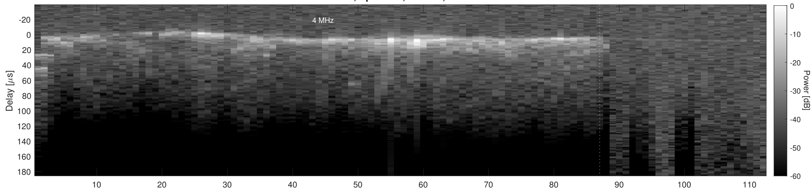
Orbit 2056, Cluttergram
