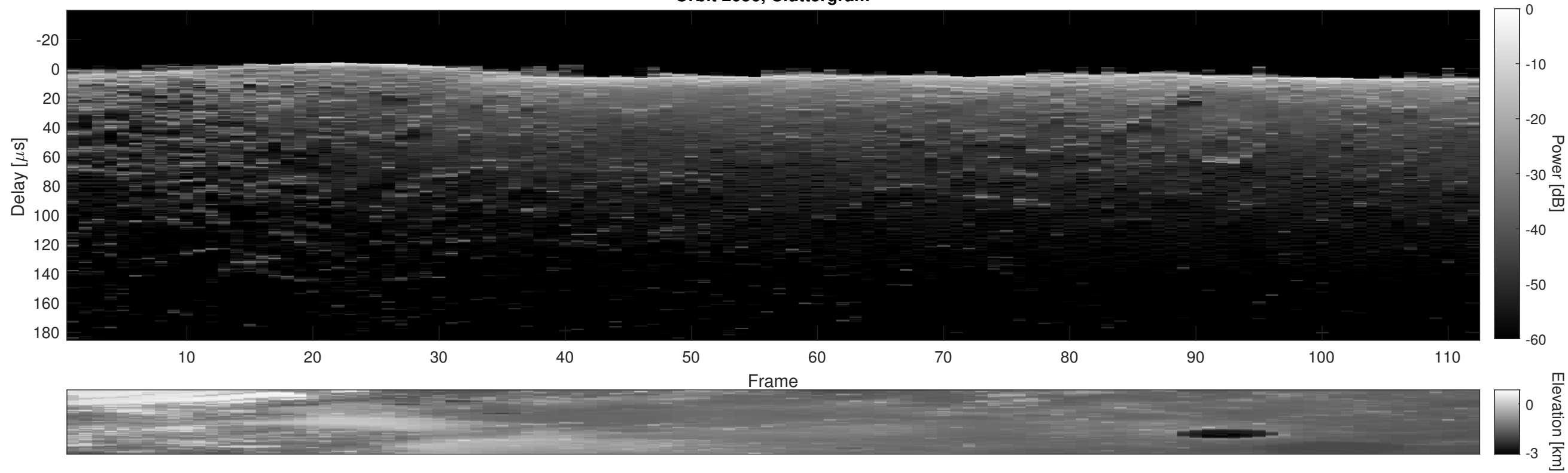
Orbit 2056, Cluttergram
