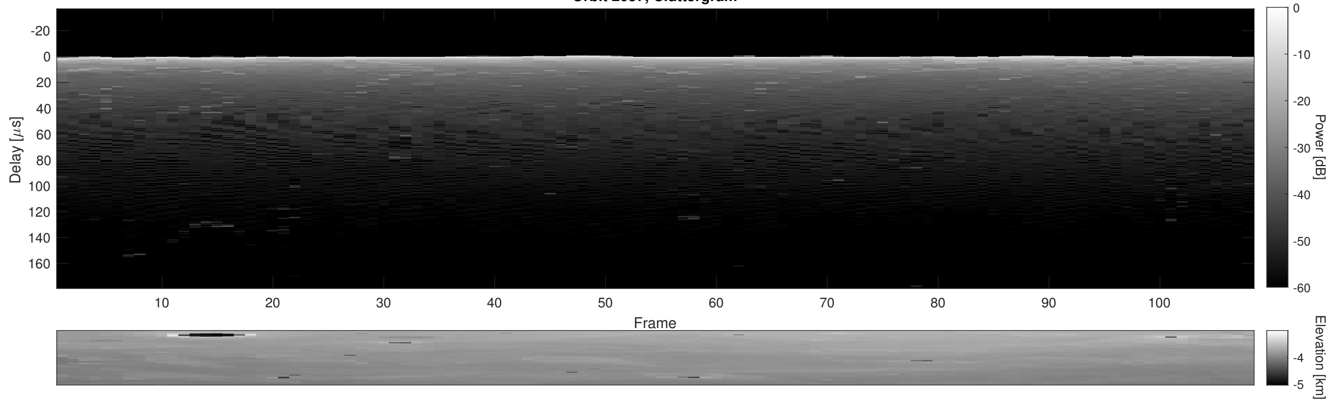
Orbit 2057, Cluttergram
