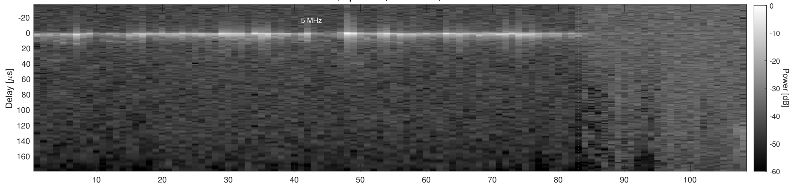
Orbit 2057, Cluttergram
