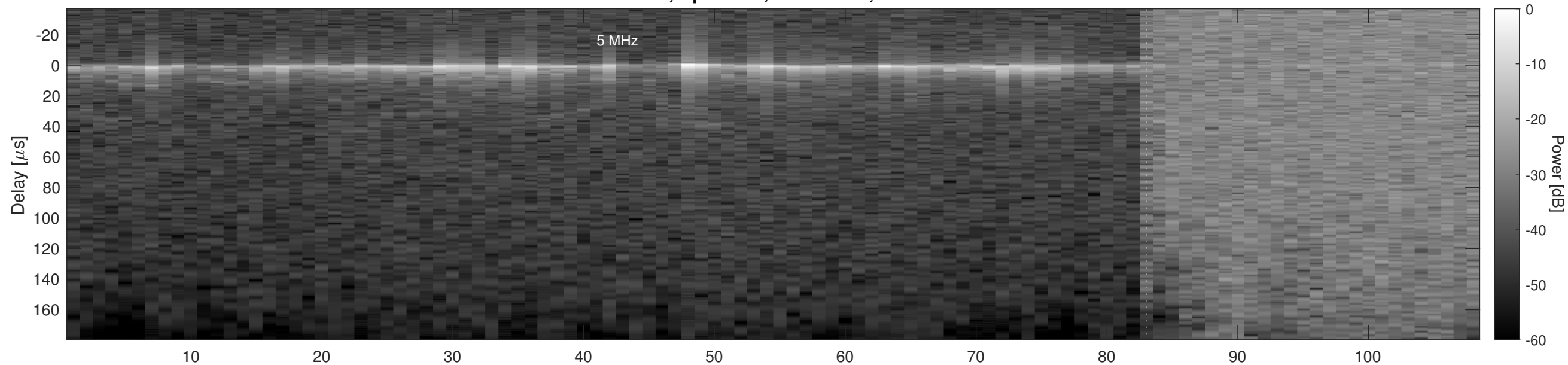
Orbit 2057, Optimized, No Window, Channel 2
