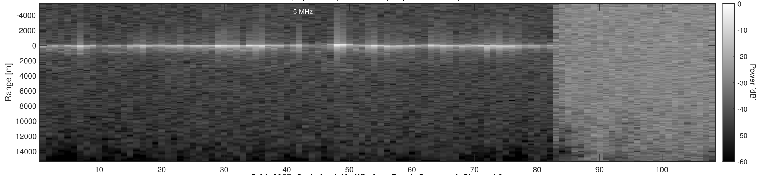
Orbit 2057, Optimized, No Window, Depth-Corrected, Channel 2
