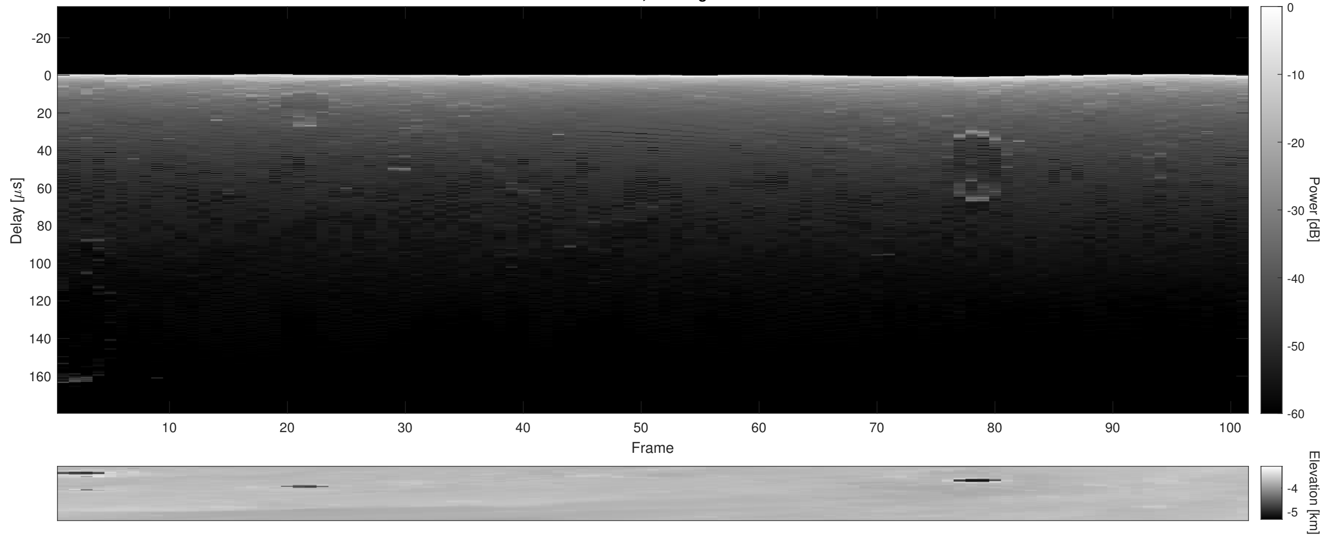
Orbit 2059, Cluttergram
