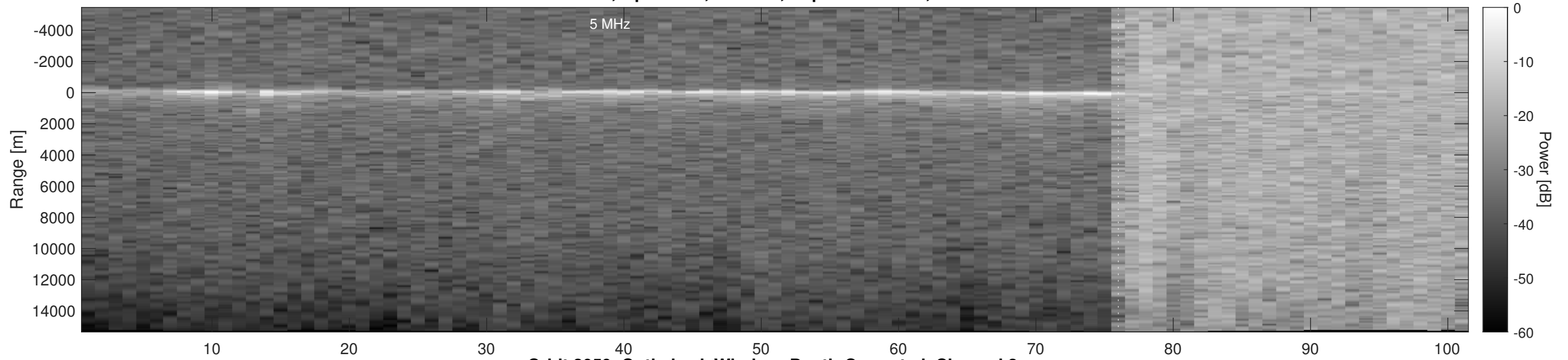
Orbit 2059, Optimized, Window, Depth-Corrected, Channel 2
