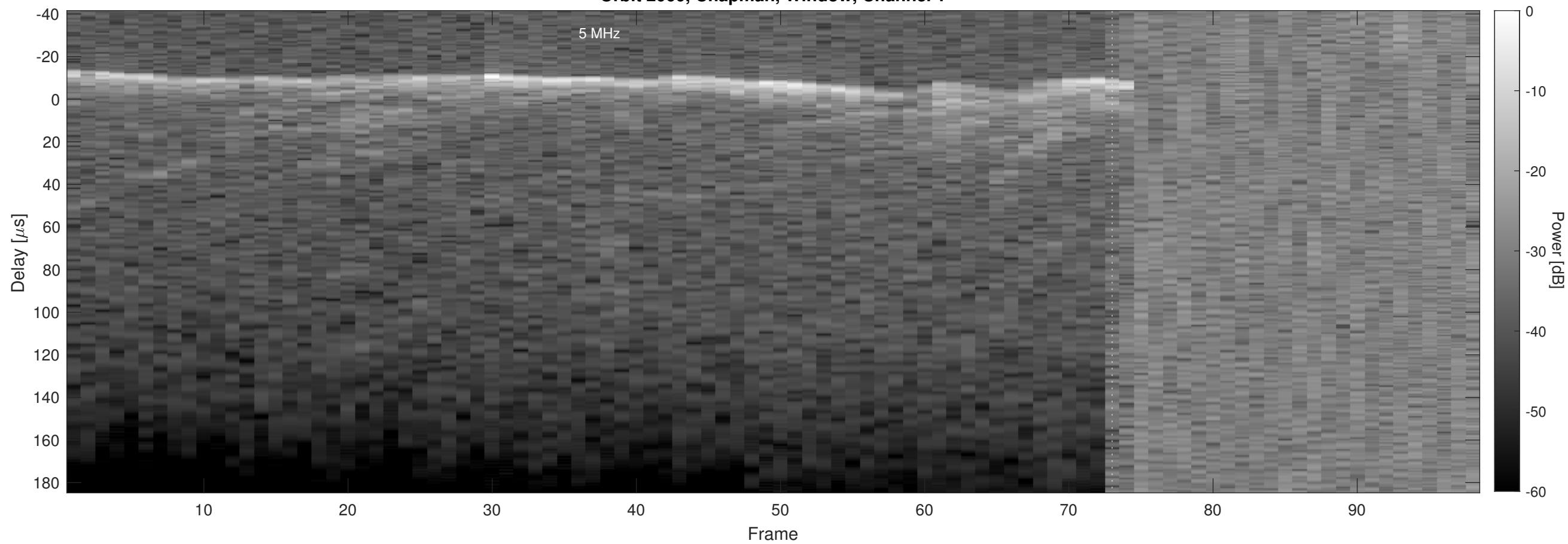
Orbit 2060, Chapman, Window, Channel 2
