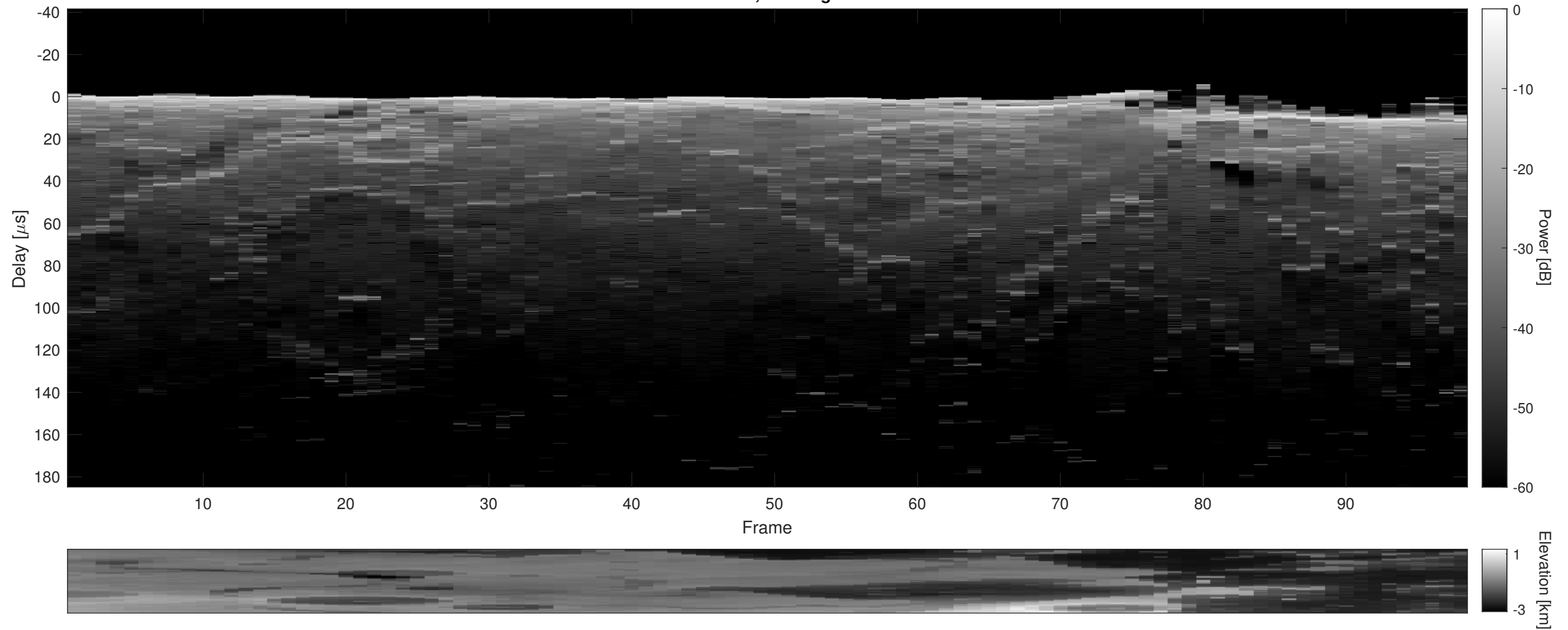
Orbit 2060, Cluttergram
