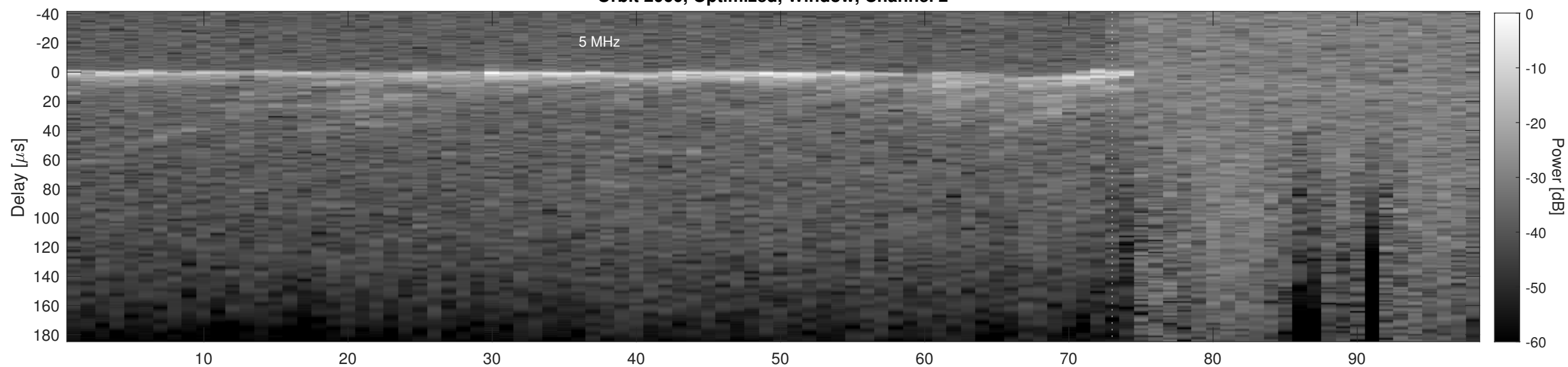
Orbit 2060, Cluttergram
