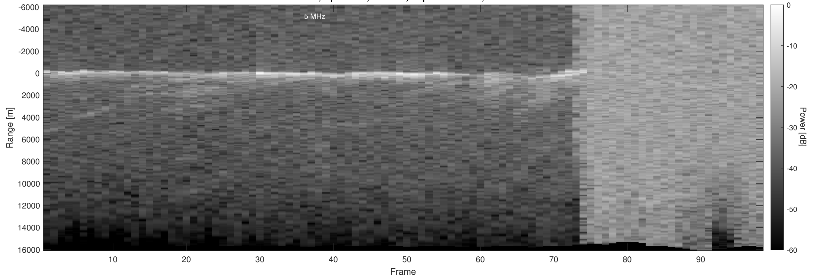
Orbit 2060, Optimized, Window, Depth-Corrected, Channel 2
