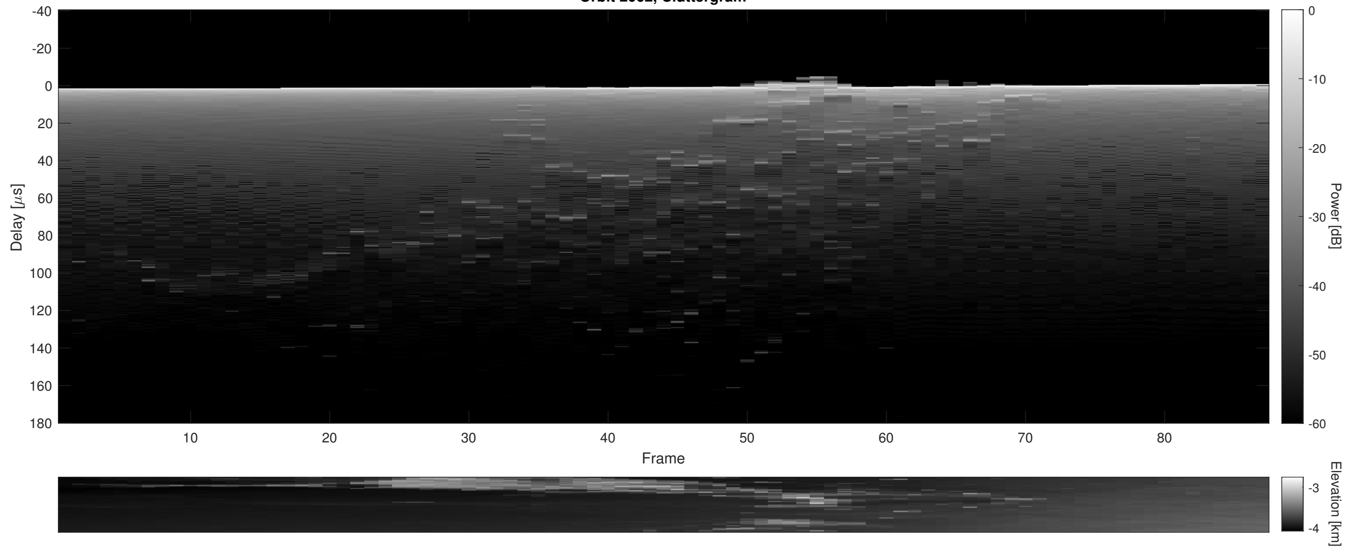
Orbit 2062, Cluttergram
