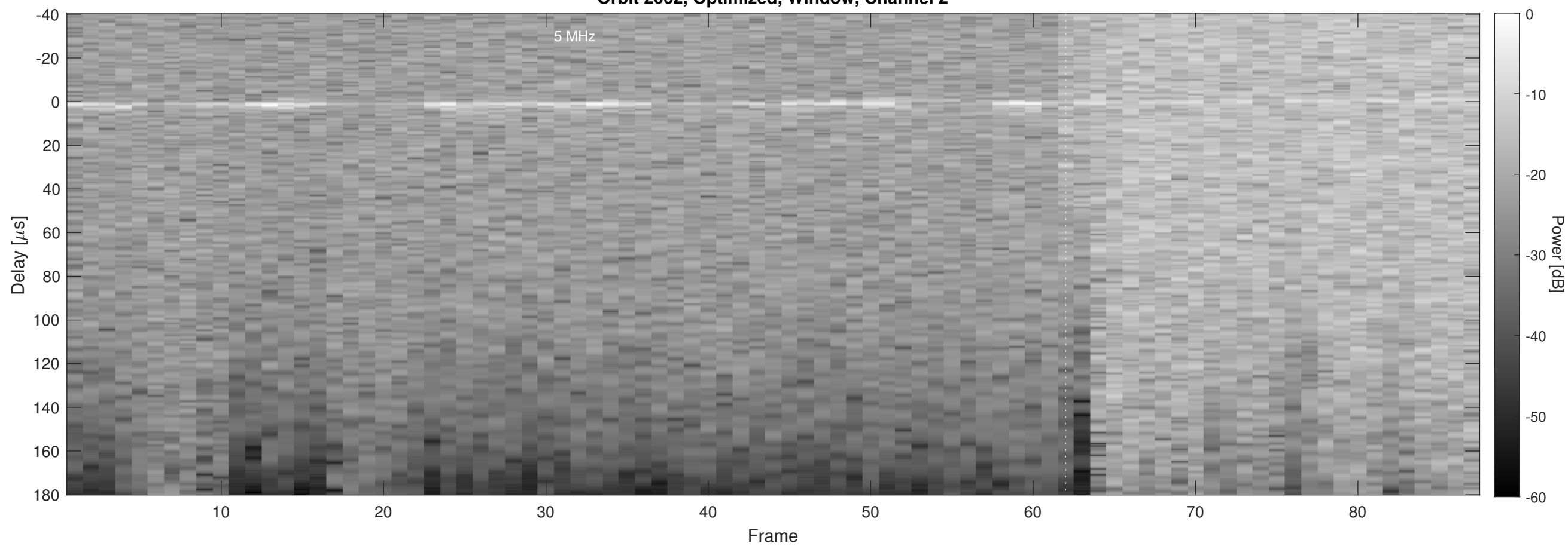
Orbit 2062, Optimized, Window, Channel 2
