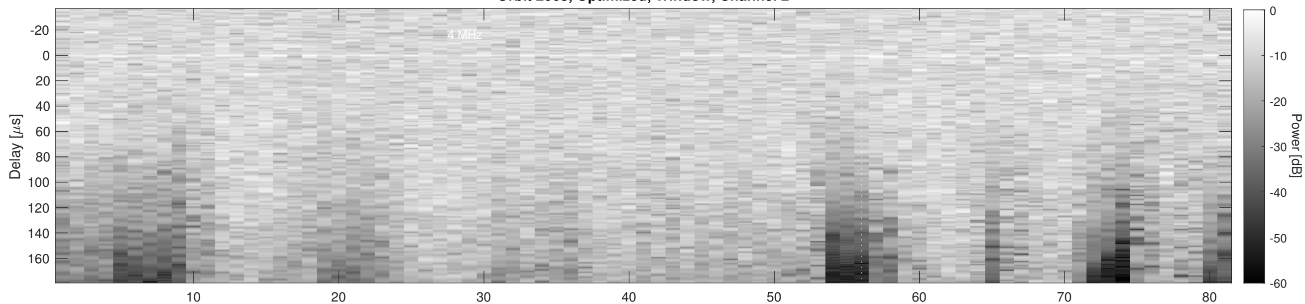
Orbit 2063, Cluttergram
