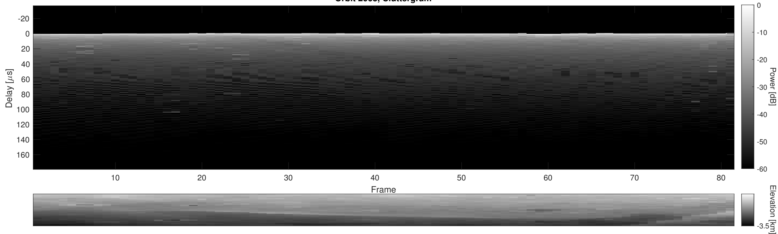
Orbit 2063, Cluttergram
