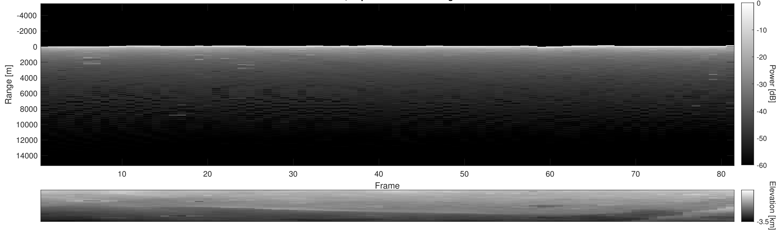
Orbit 2063, Depth-Corrected Cluttergram
