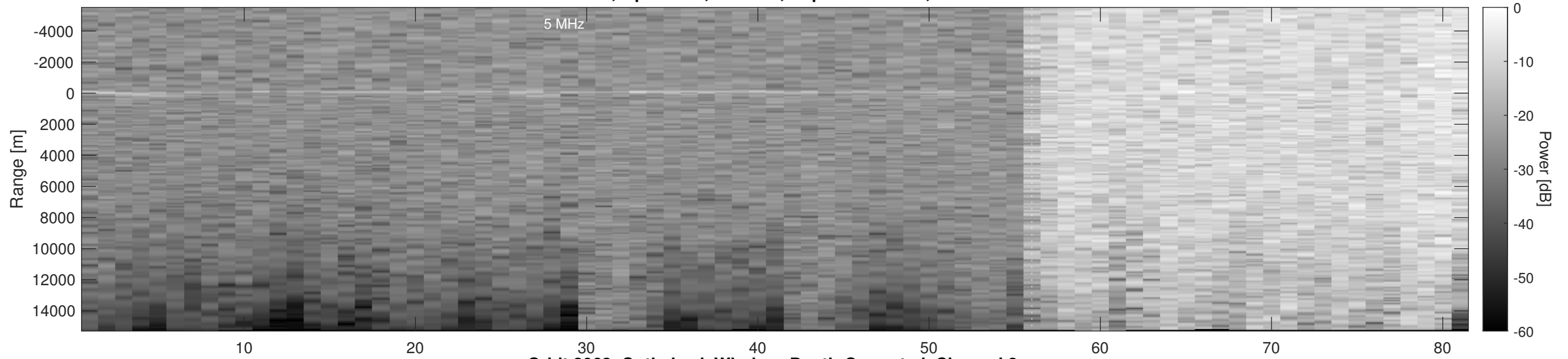
Orbit 2063, Optimized, Window, Depth-Corrected, Channel 2
