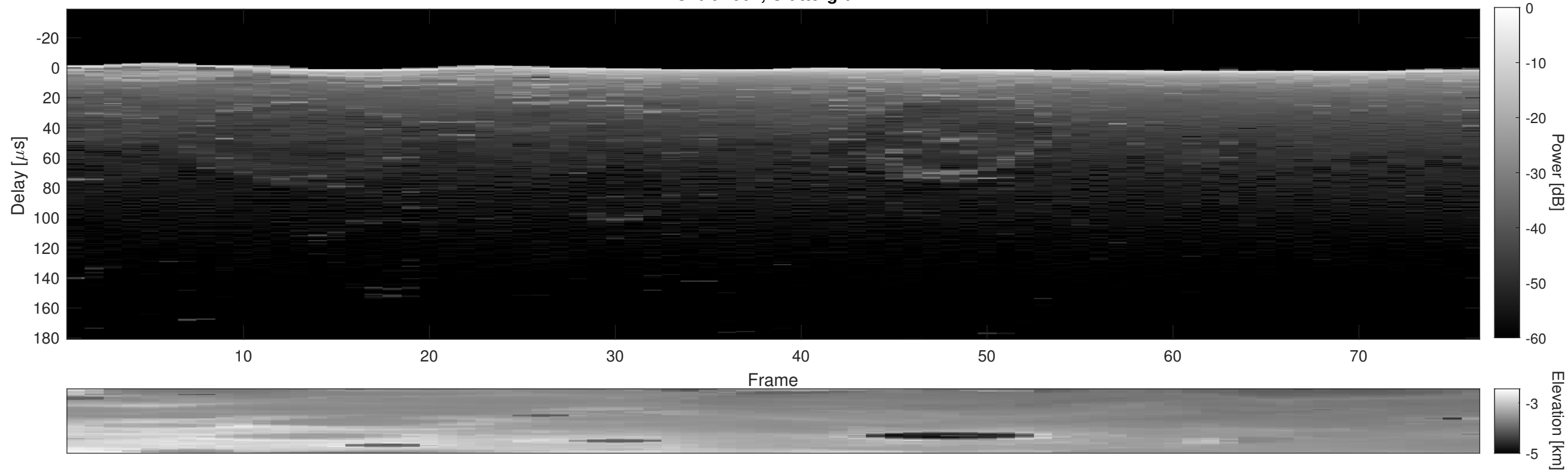
Orbit 2064, Cluttergram
