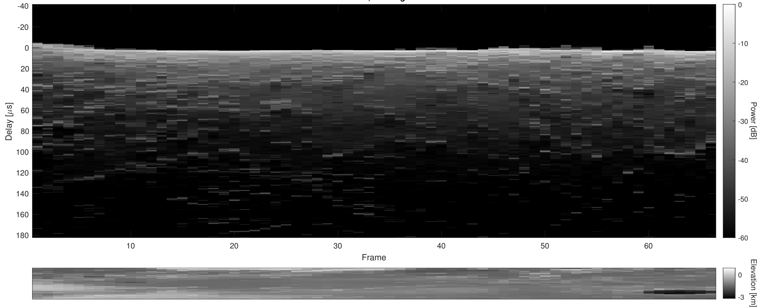
Orbit 2067, Cluttergram
