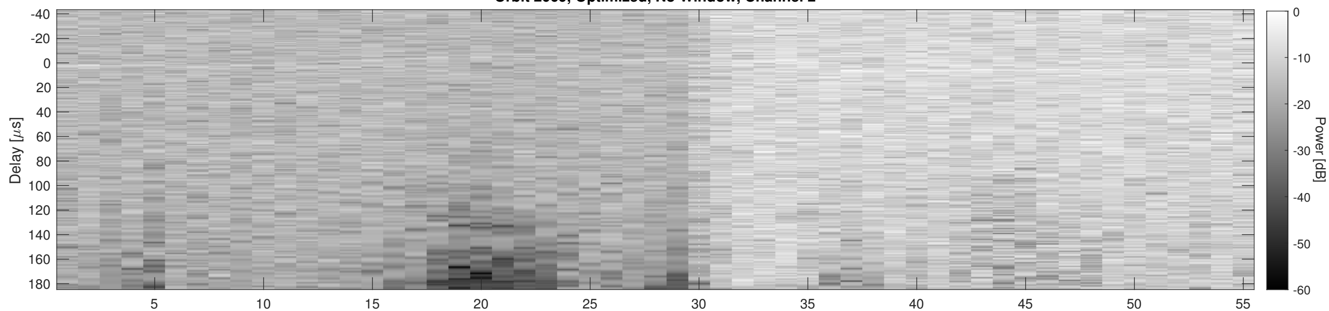
Orbit 2069, Cluttergram
