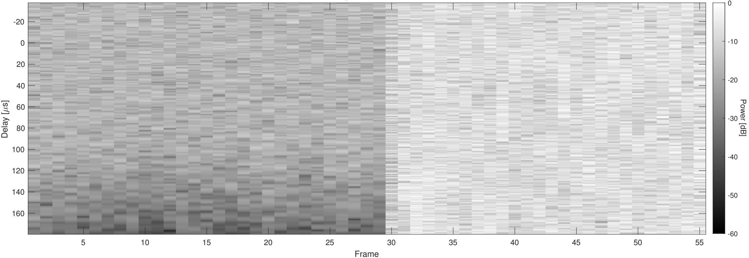
Orbit 2070, Chapman, Window, Channel 2
