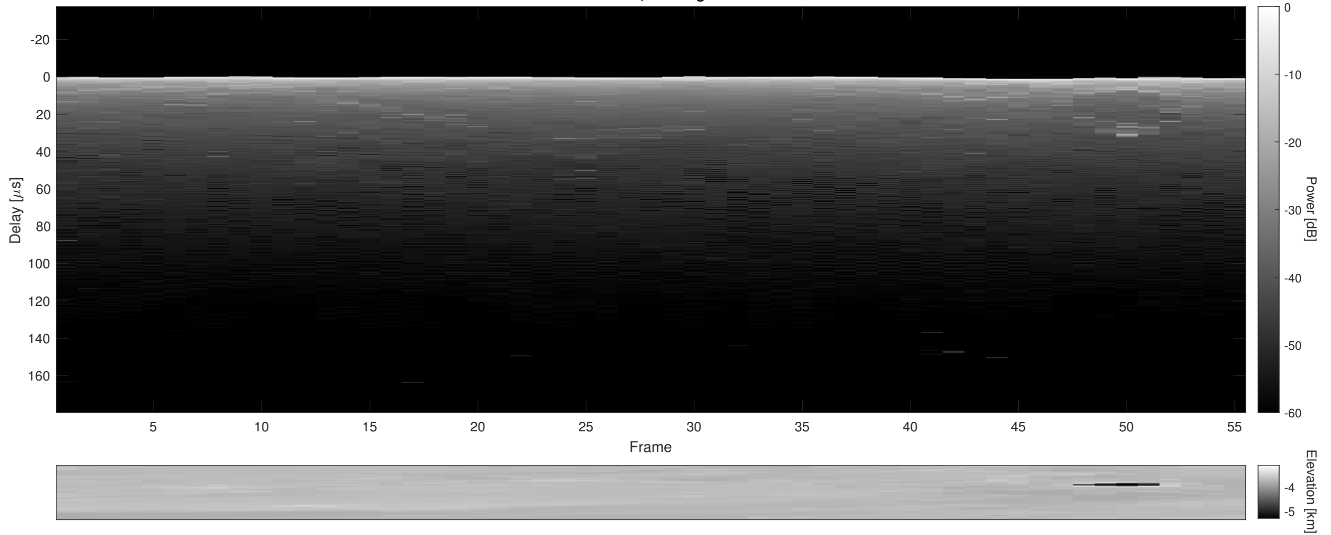
Orbit 2070, Cluttergram
