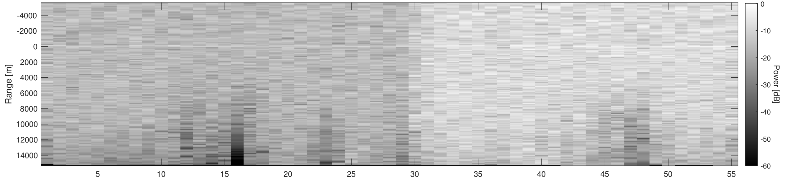
Orbit 2070, Depth-Corrected Cluttergram
