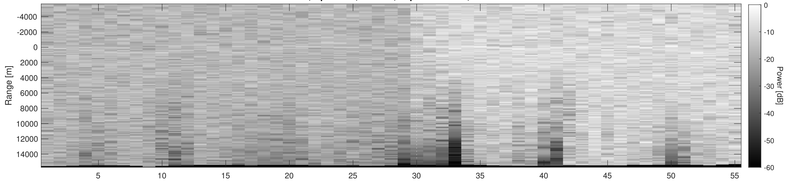
Orbit 2071, Depth-Corrected Cluttergram
