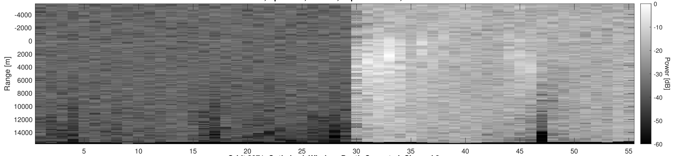
Orbit 2071, Optimized, Window, Depth-Corrected, Channel 2
