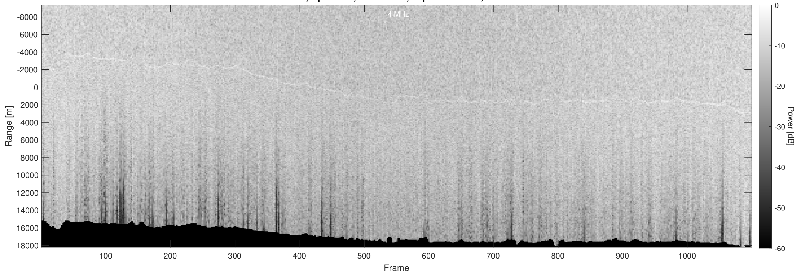
Orbit 2086, Optimized, No Window, Depth-Corrected, Channel 2
