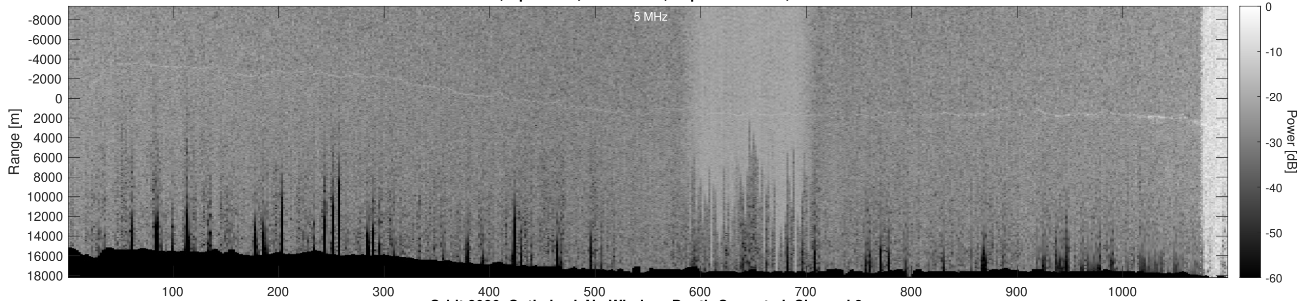
Orbit 2086, Optimized, No Window, Depth-Corrected, Channel 2
