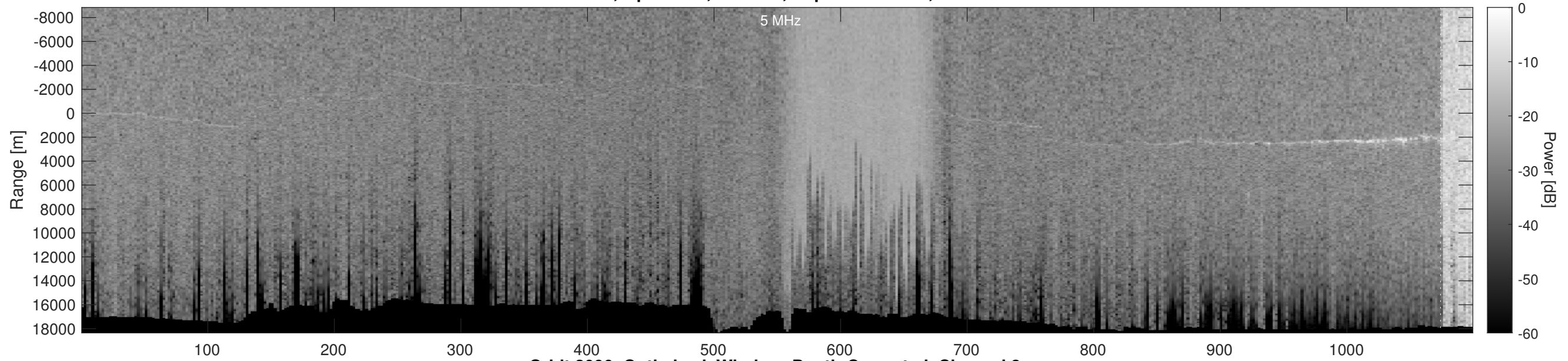
Orbit 2090, Optimized, Window, Depth-Corrected, Channel 2
