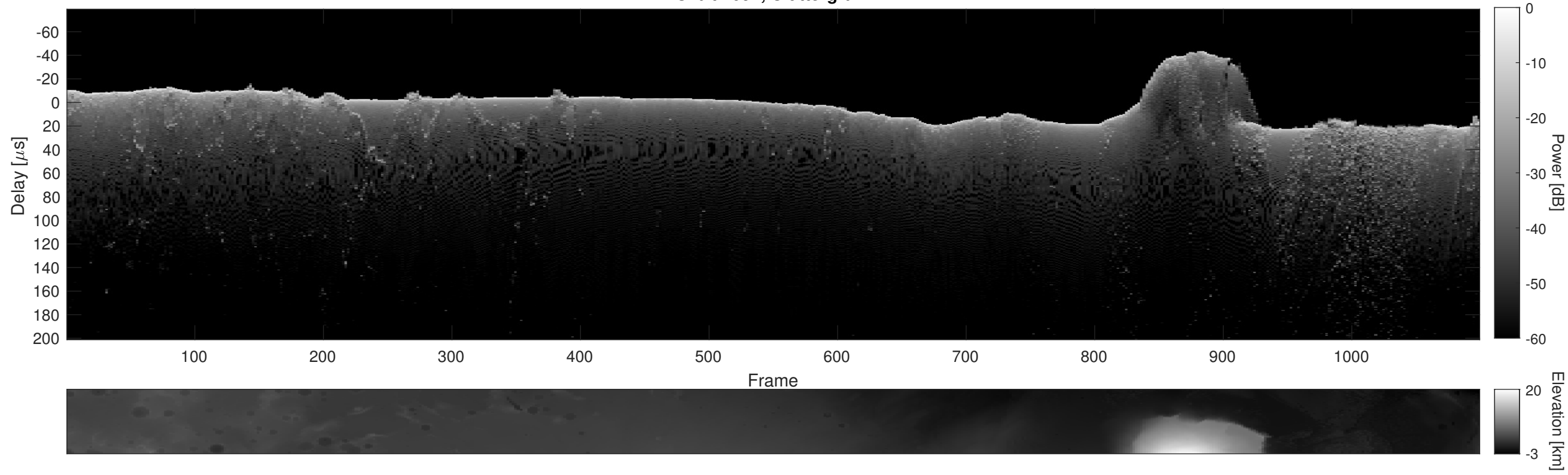
Orbit 2091, Cluttergram
