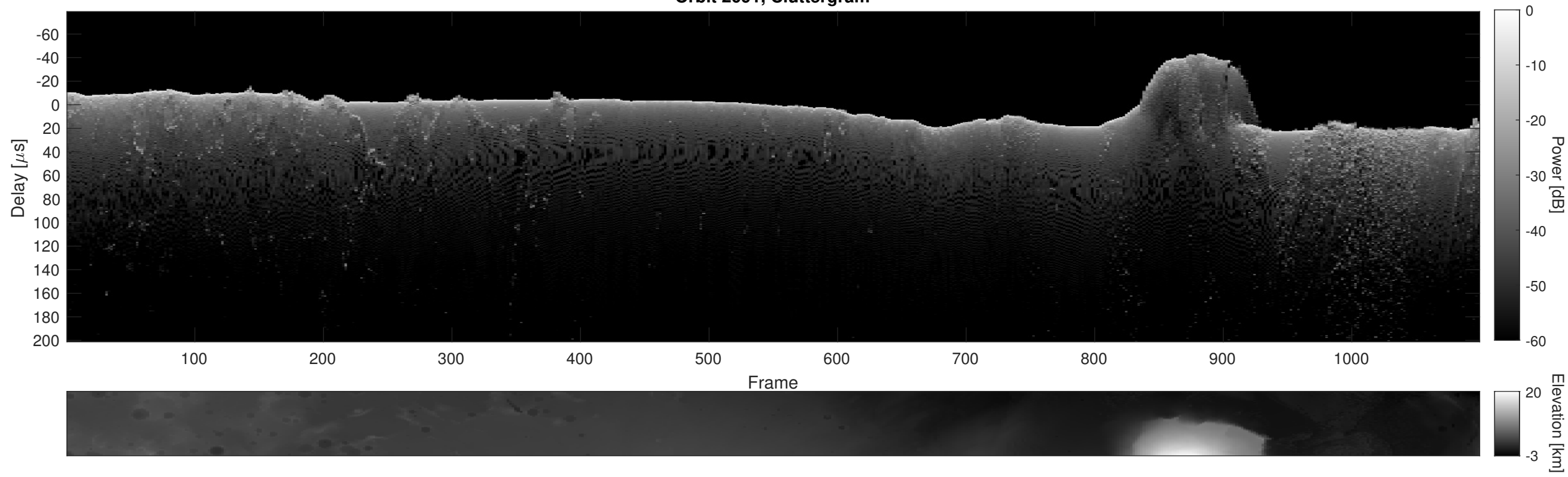
Orbit 2091, Cluttergram
