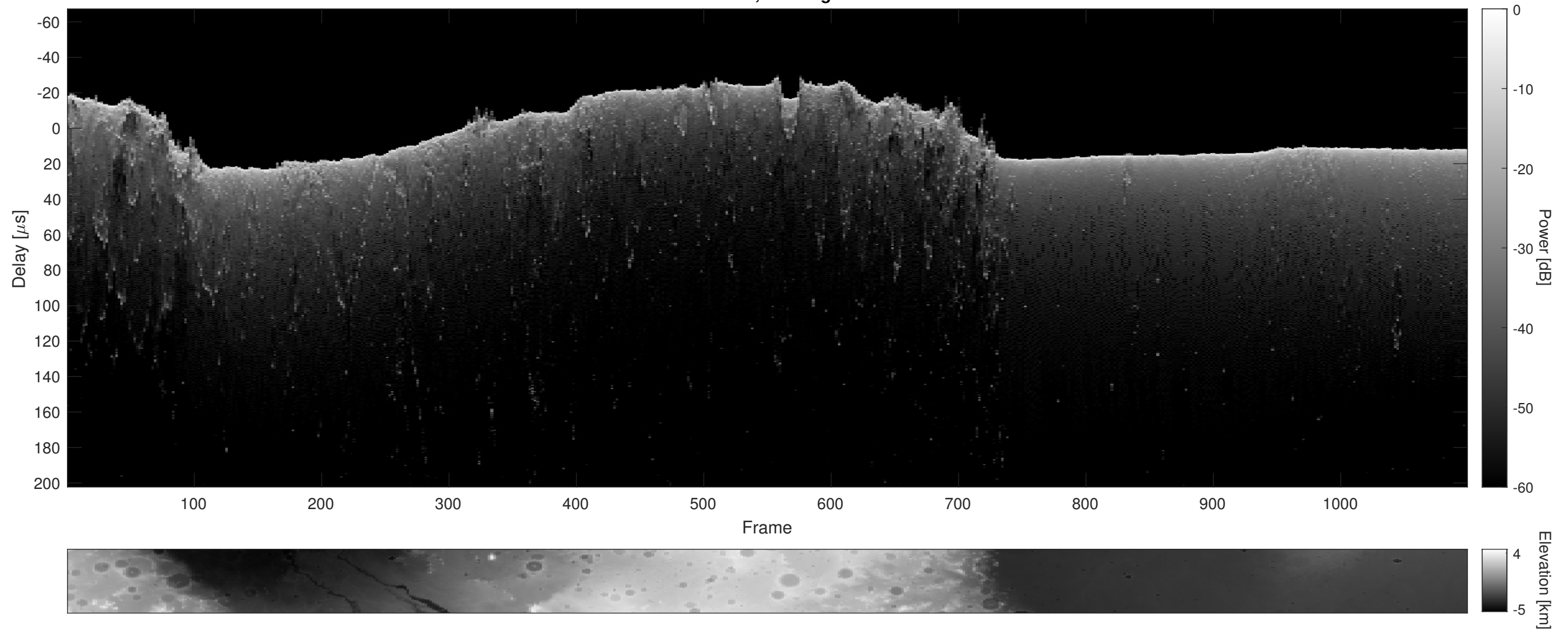
Orbit 2107, Cluttergram
