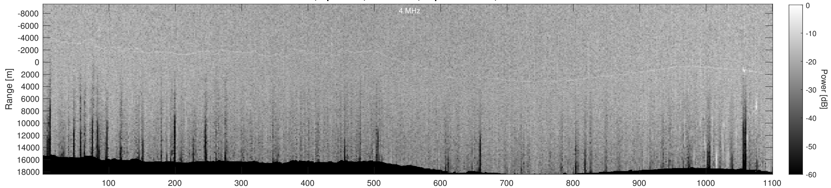
Orbit 2110, Depth-Corrected Cluttergram
