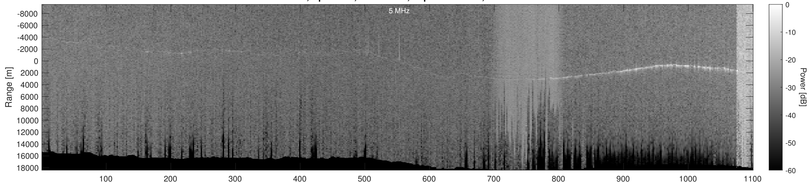
Orbit 2110, Optimized, No Window, Depth-Corrected, Channel 2
