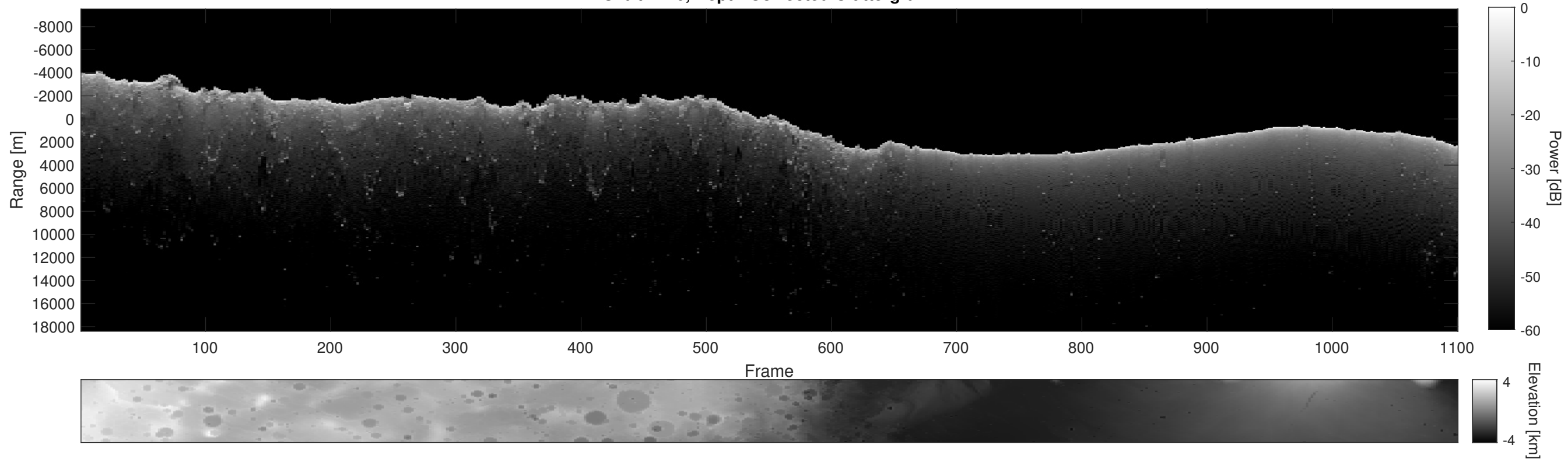
Orbit 2110, Depth-Corrected Cluttergram
