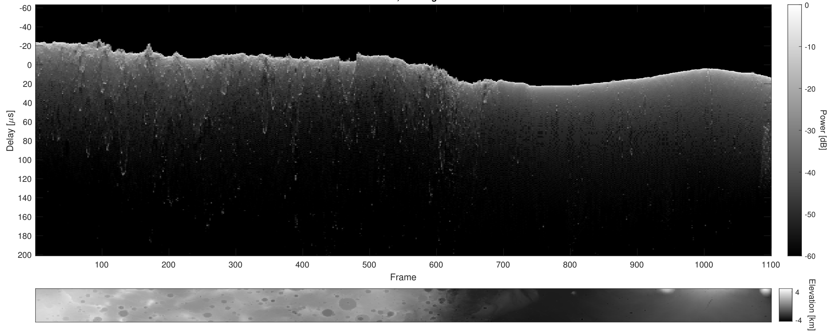
Orbit 2121, Cluttergram
