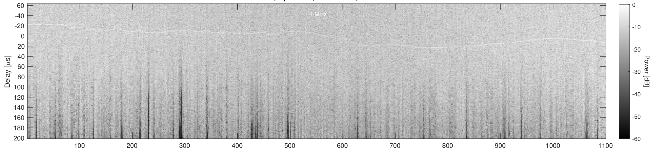
Orbit 2121, Cluttergram
