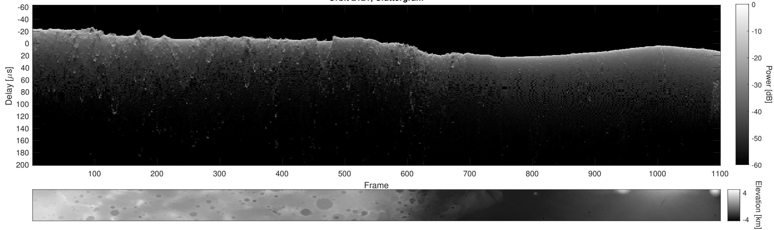
Orbit 2121, Cluttergram
