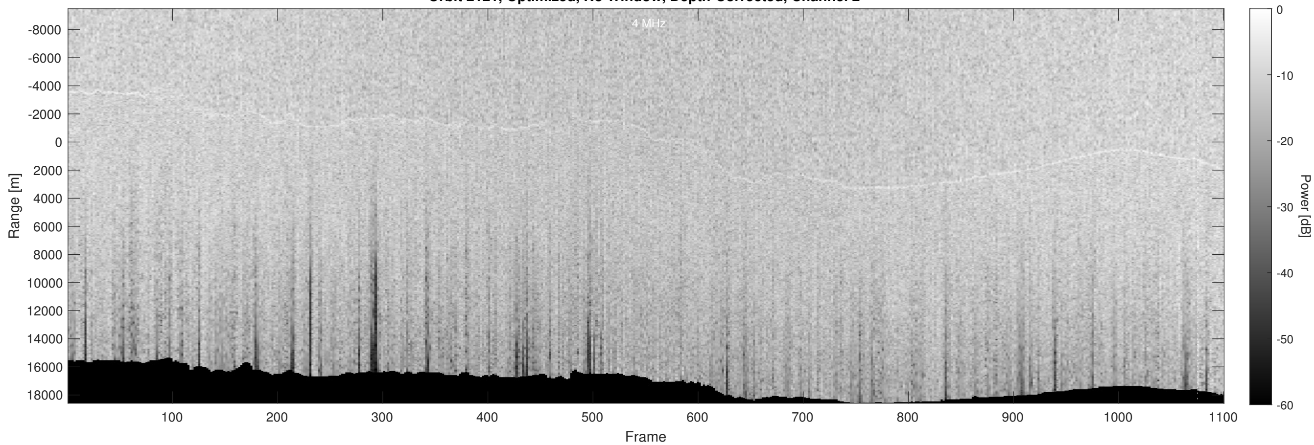
Orbit 2121, Optimized, No Window, Depth-Corrected, Channel 2
