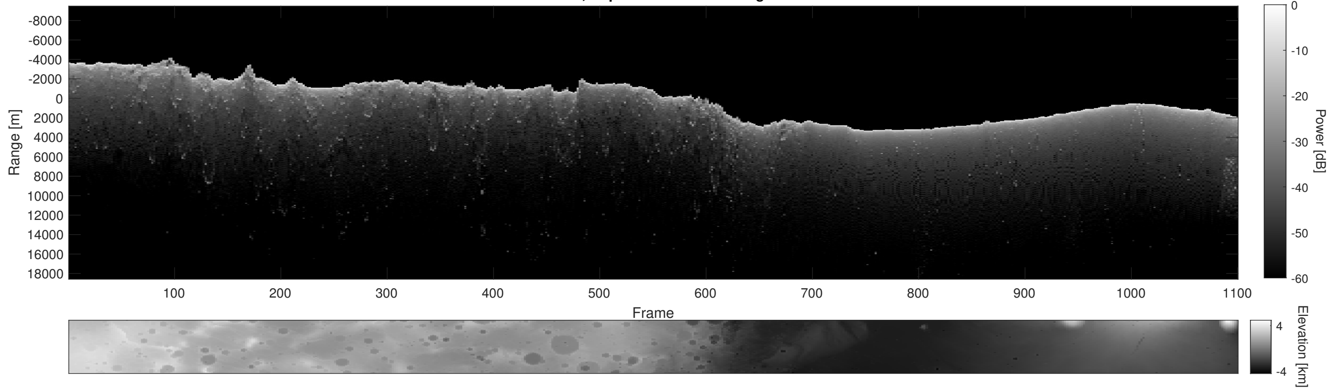
Orbit 2121, Depth-Corrected Cluttergram
