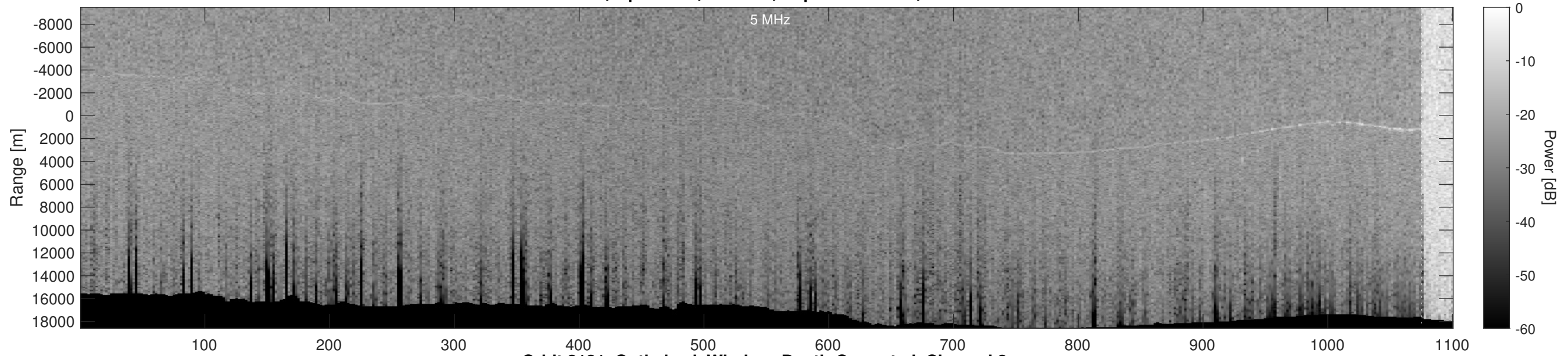
Orbit 2121, Optimized, Window, Depth-Corrected, Channel 2
