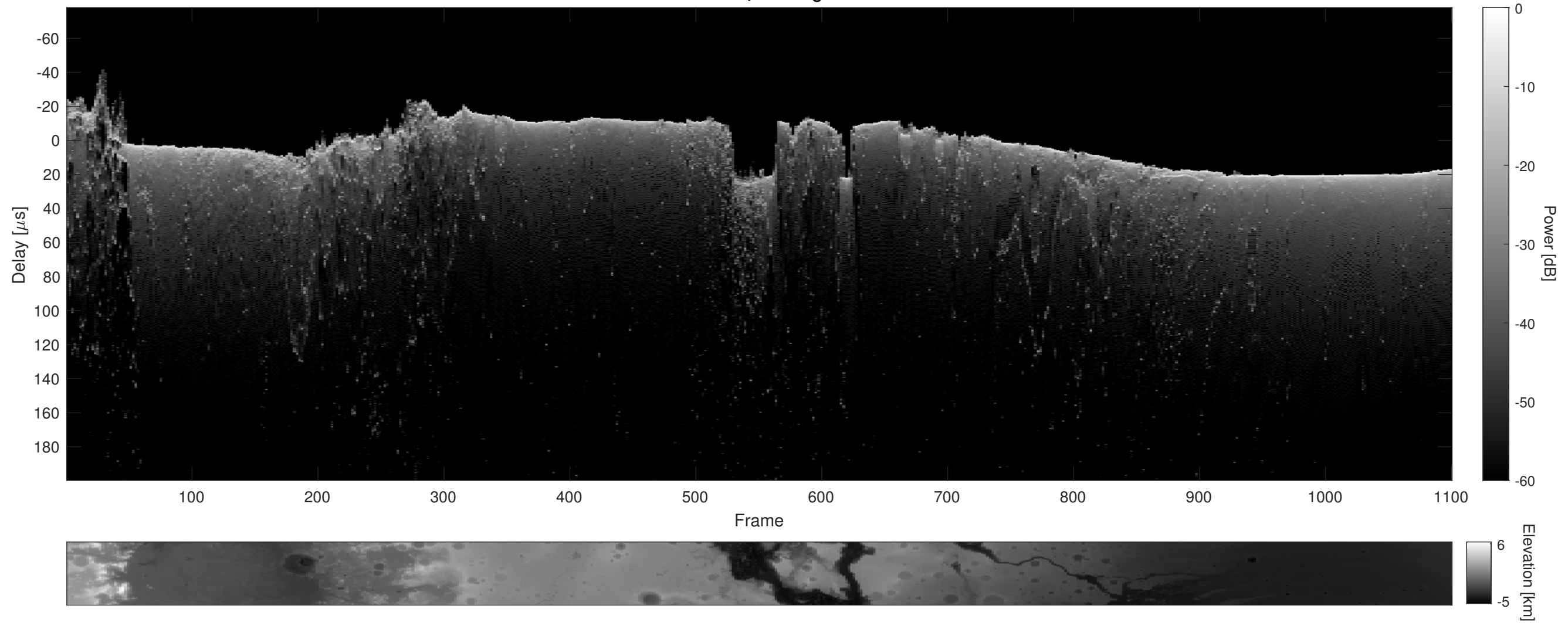
Orbit 2123, Cluttergram
