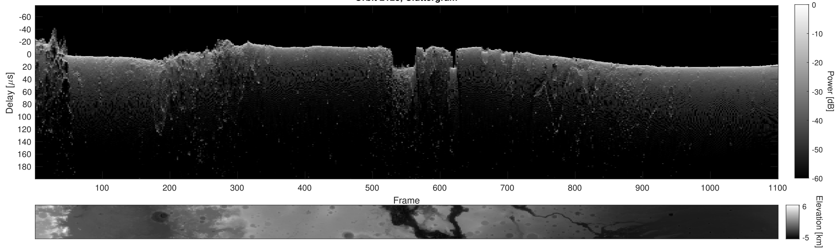
Orbit 2123, Cluttergram
