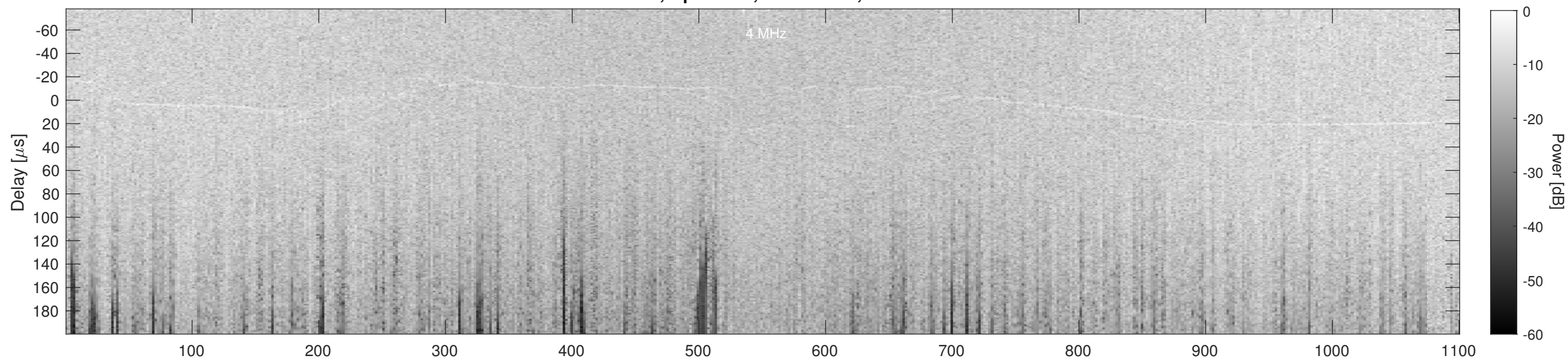
Orbit 2123, Cluttergram
