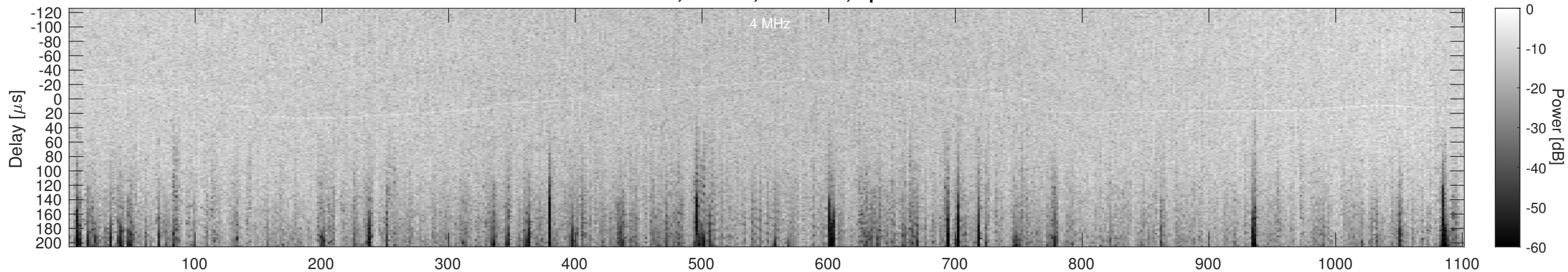
Orbit 2129, Cluttergram
