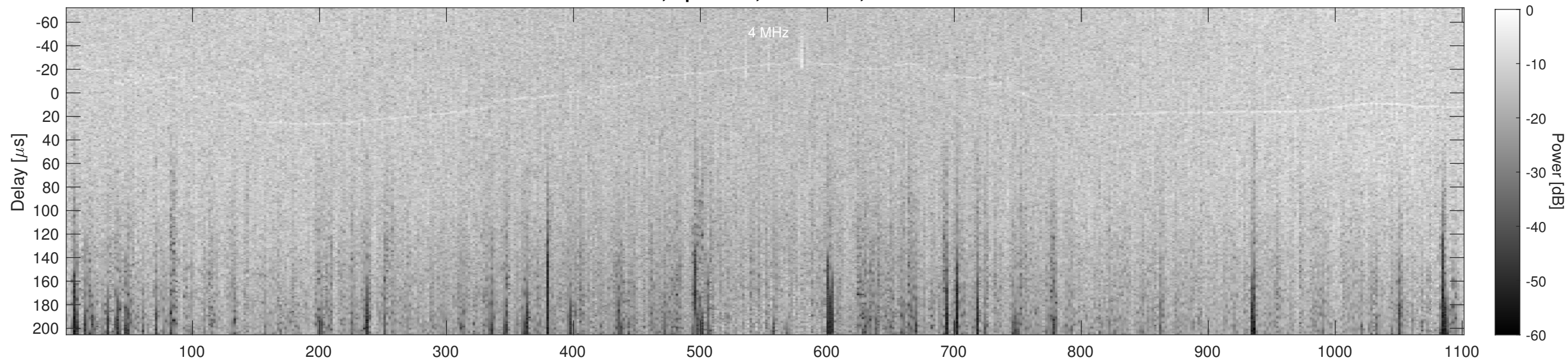
Orbit 2129, Cluttergram
