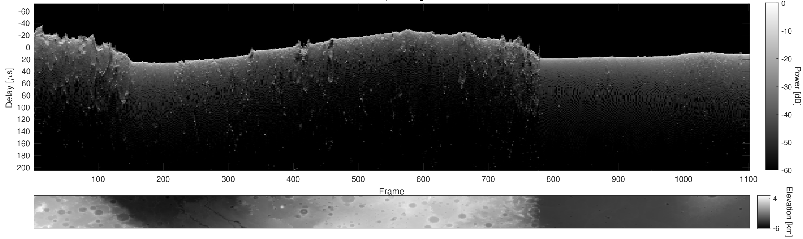
Orbit 2129, Cluttergram
