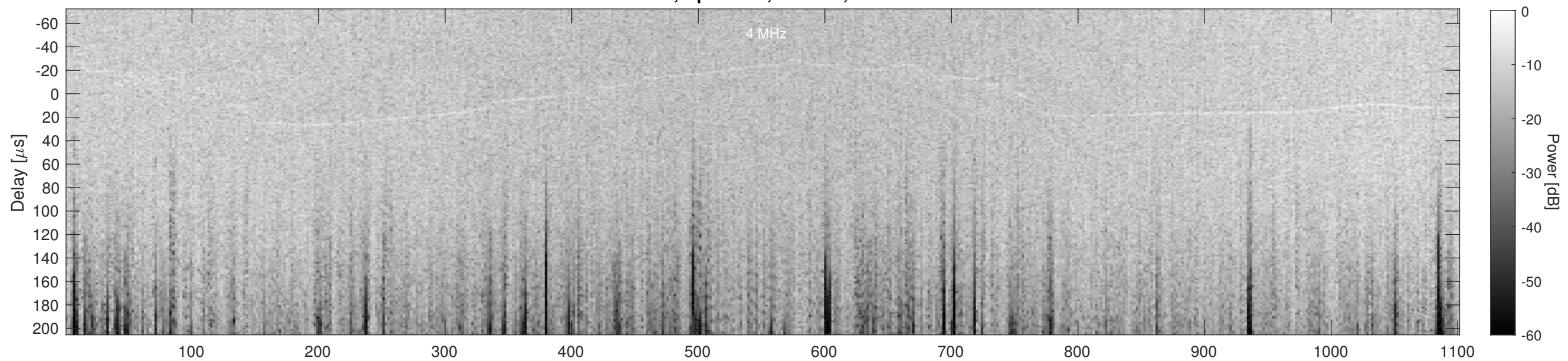
Orbit 2129, Cluttergram
