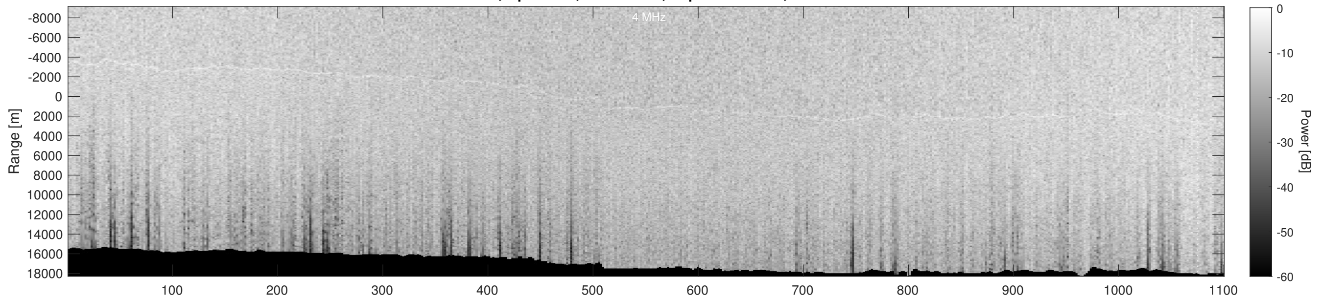
Orbit 2130, Depth-Corrected Cluttergram
