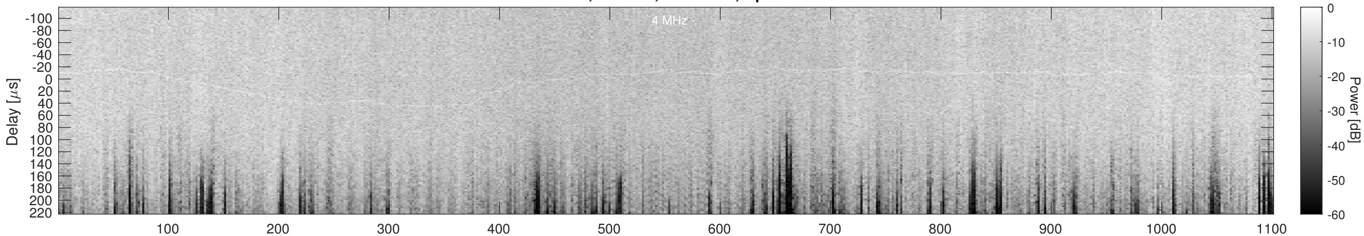
Orbit 2144, Cluttergram
