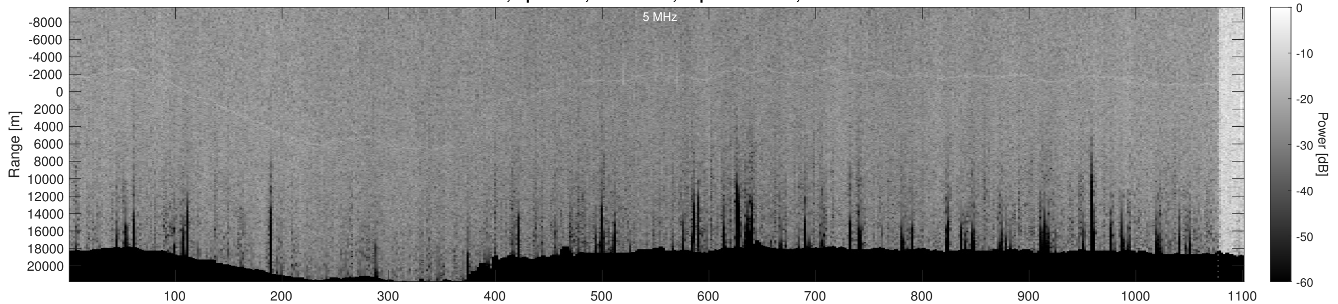
Orbit 2144, Optimized, No Window, Depth-Corrected, Channel 2
