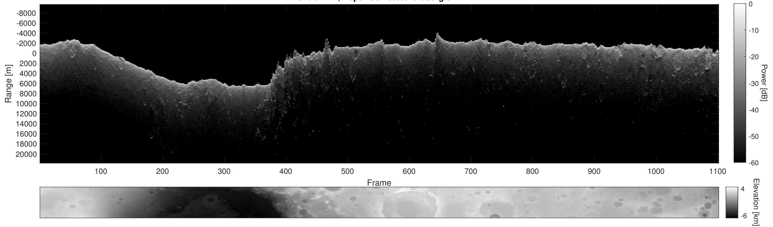
Orbit 2144, Depth-Corrected Cluttergram
