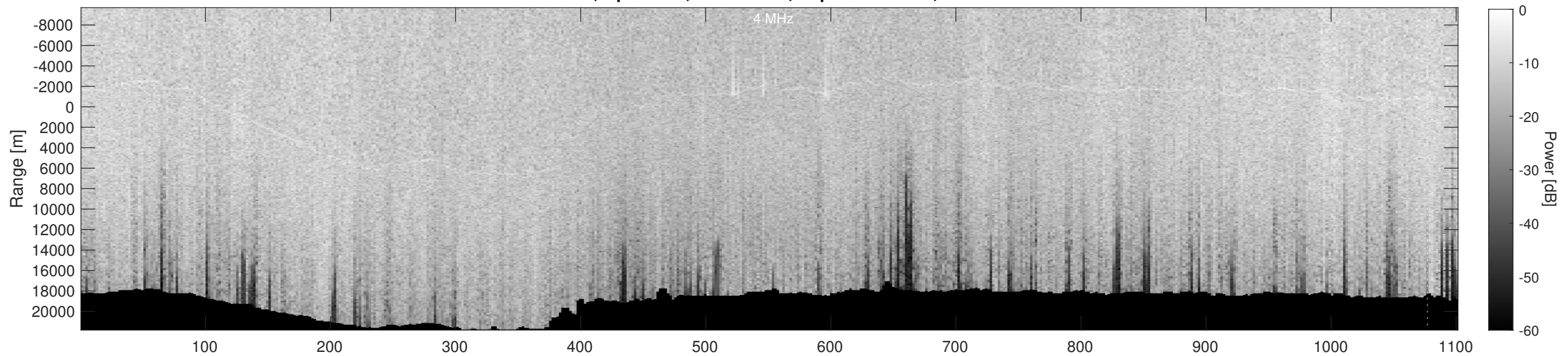
Orbit 2144, Depth-Corrected Cluttergram
