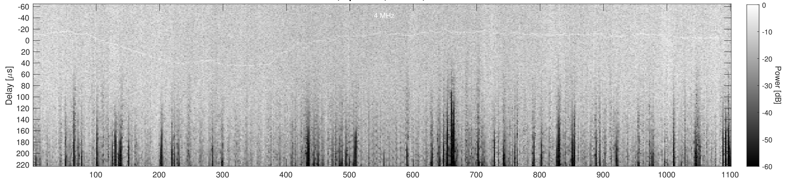
Orbit 2144, Cluttergram
