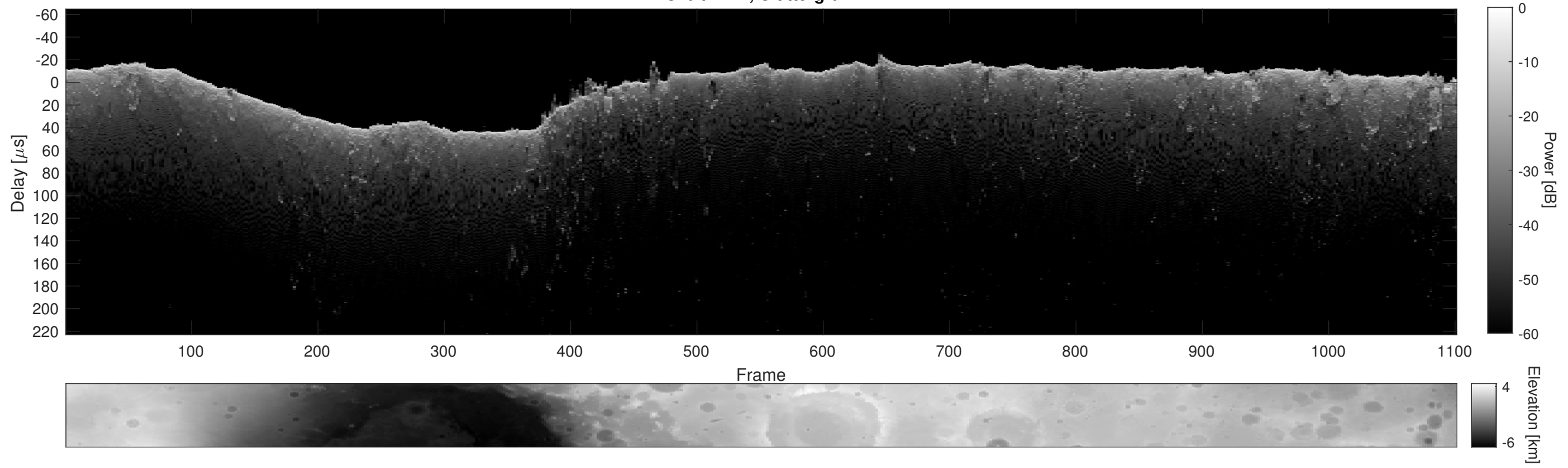
Orbit 2144, Cluttergram
