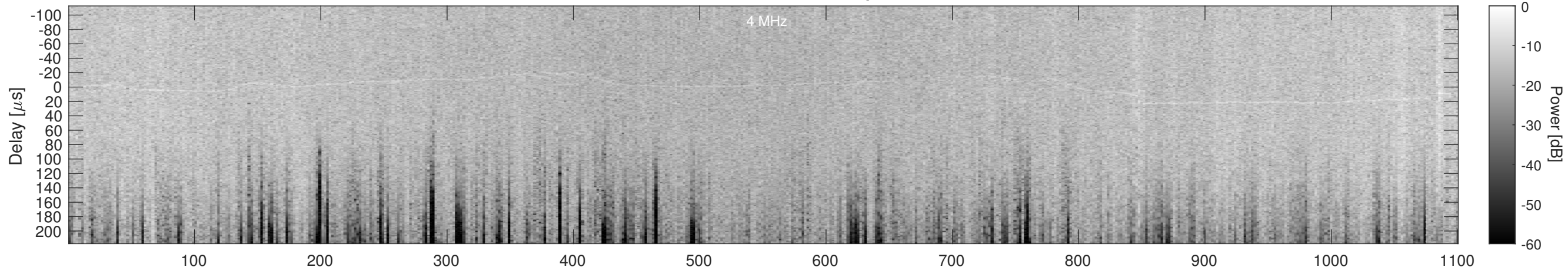
Orbit 2149, Cluttergram
