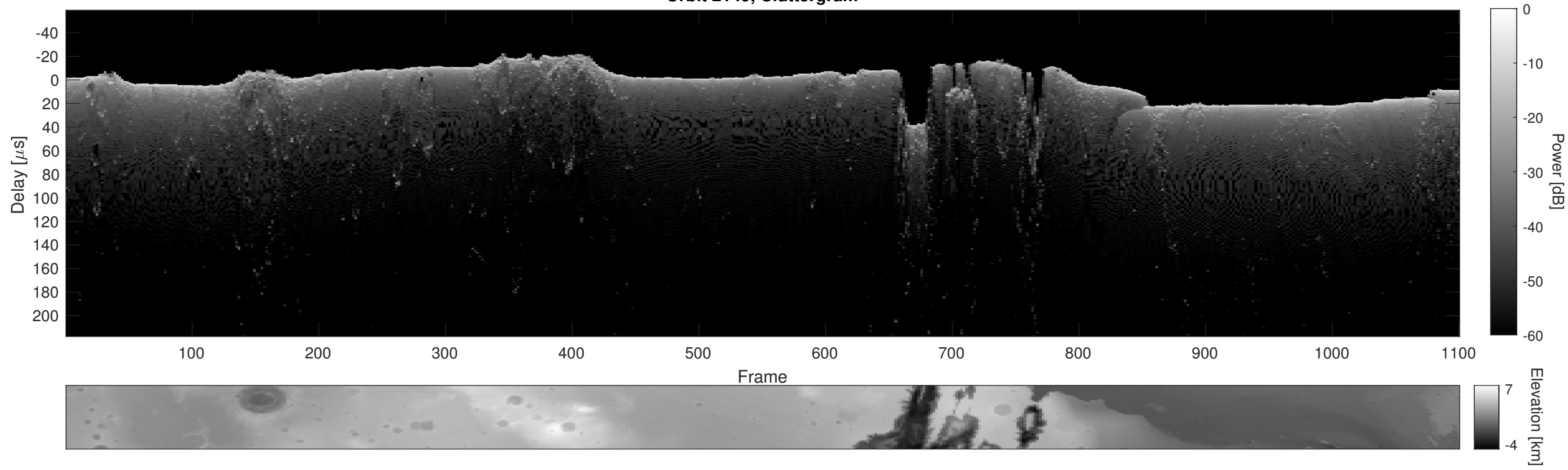
Orbit 2149, Cluttergram
