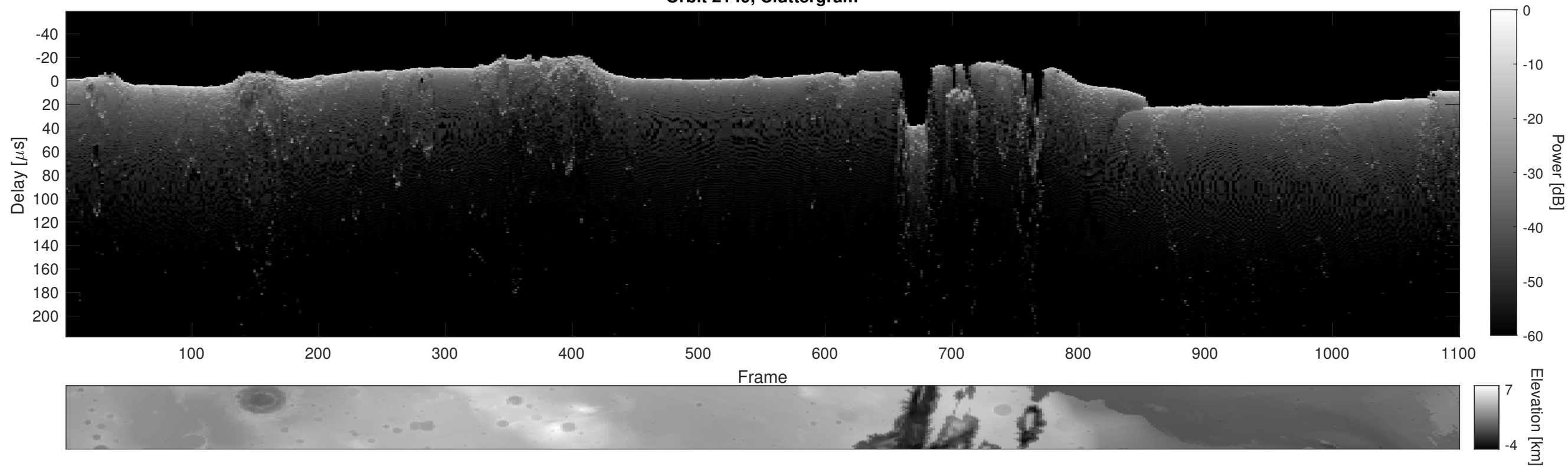
Orbit 2149, Cluttergram
