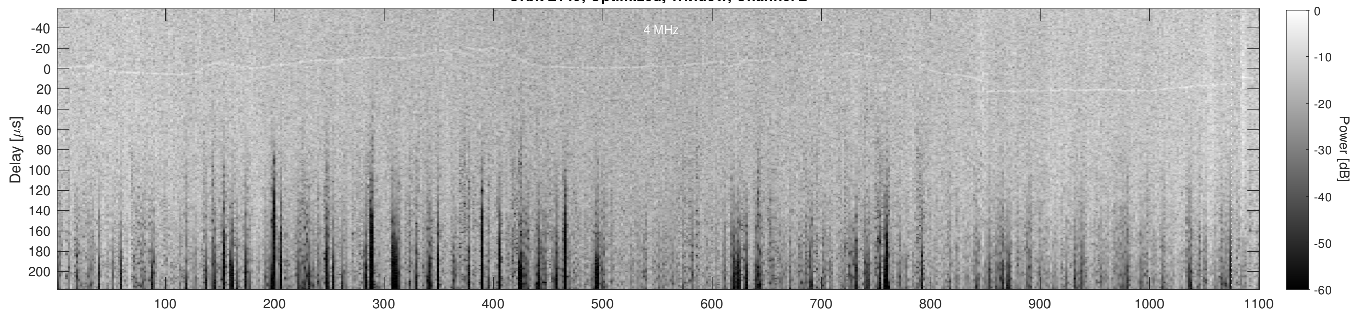
Orbit 2149, Cluttergram
