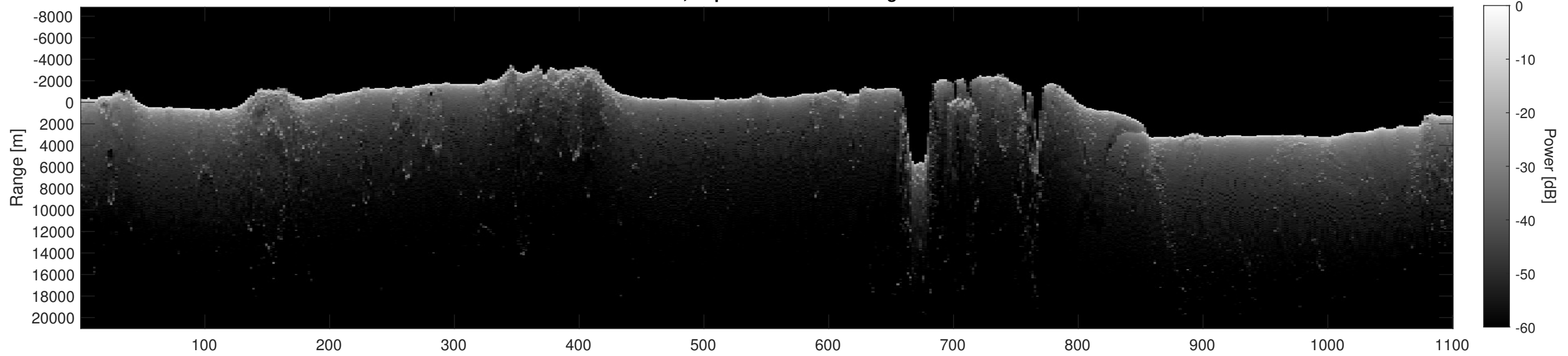
Orbit 2149, Depth-Corrected Cluttergram
