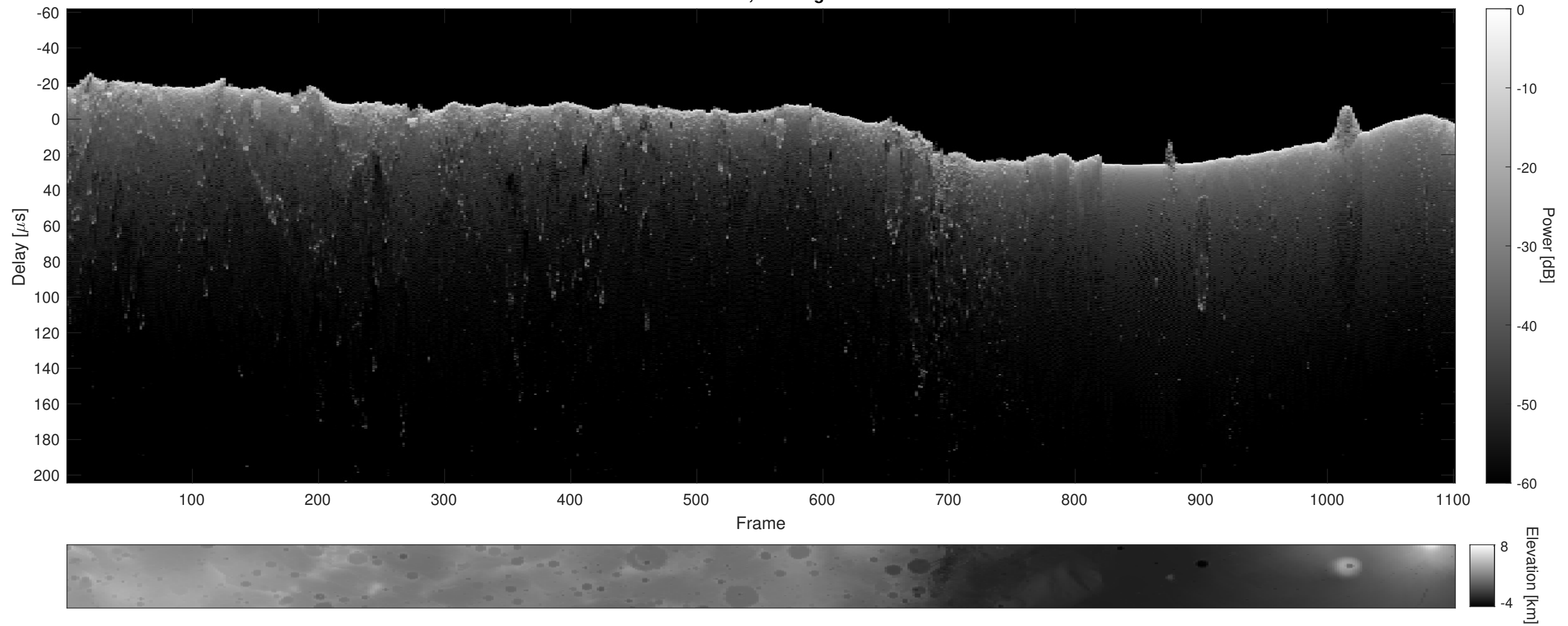
Orbit 2154, Cluttergram
