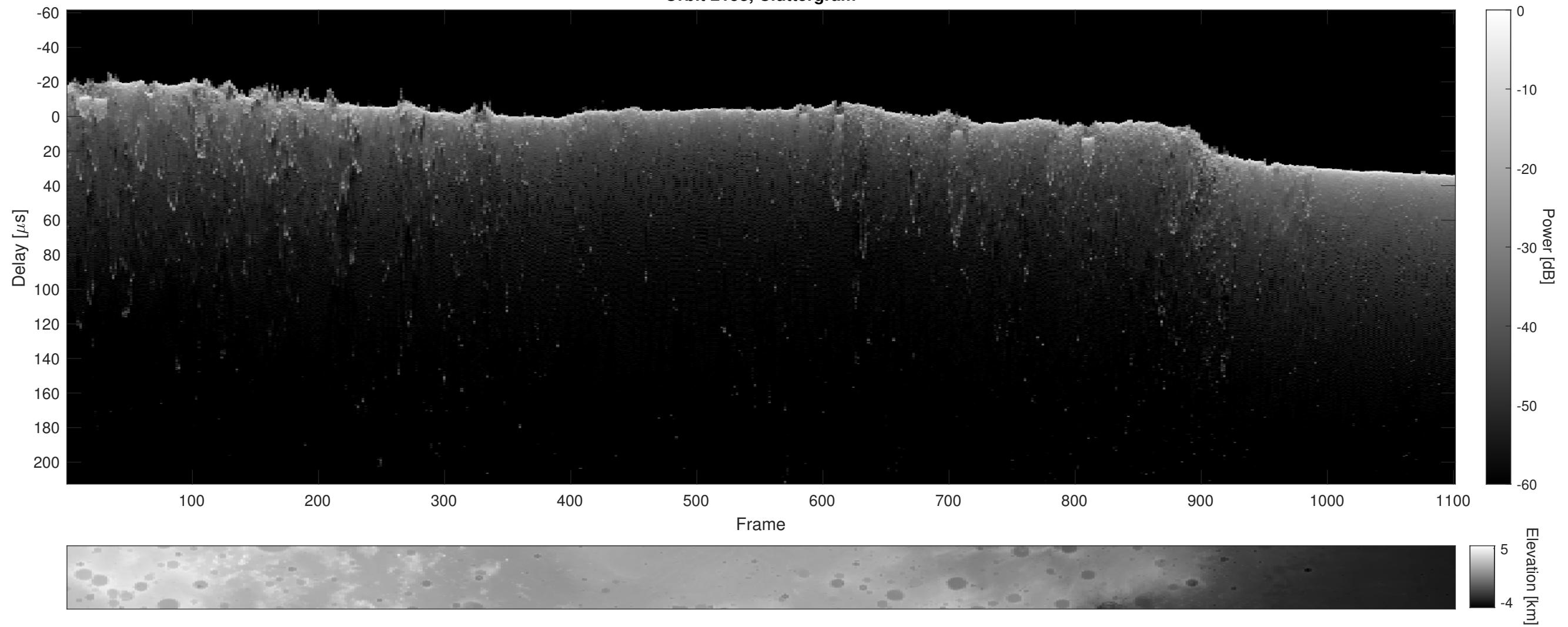
Orbit 2158, Cluttergram
