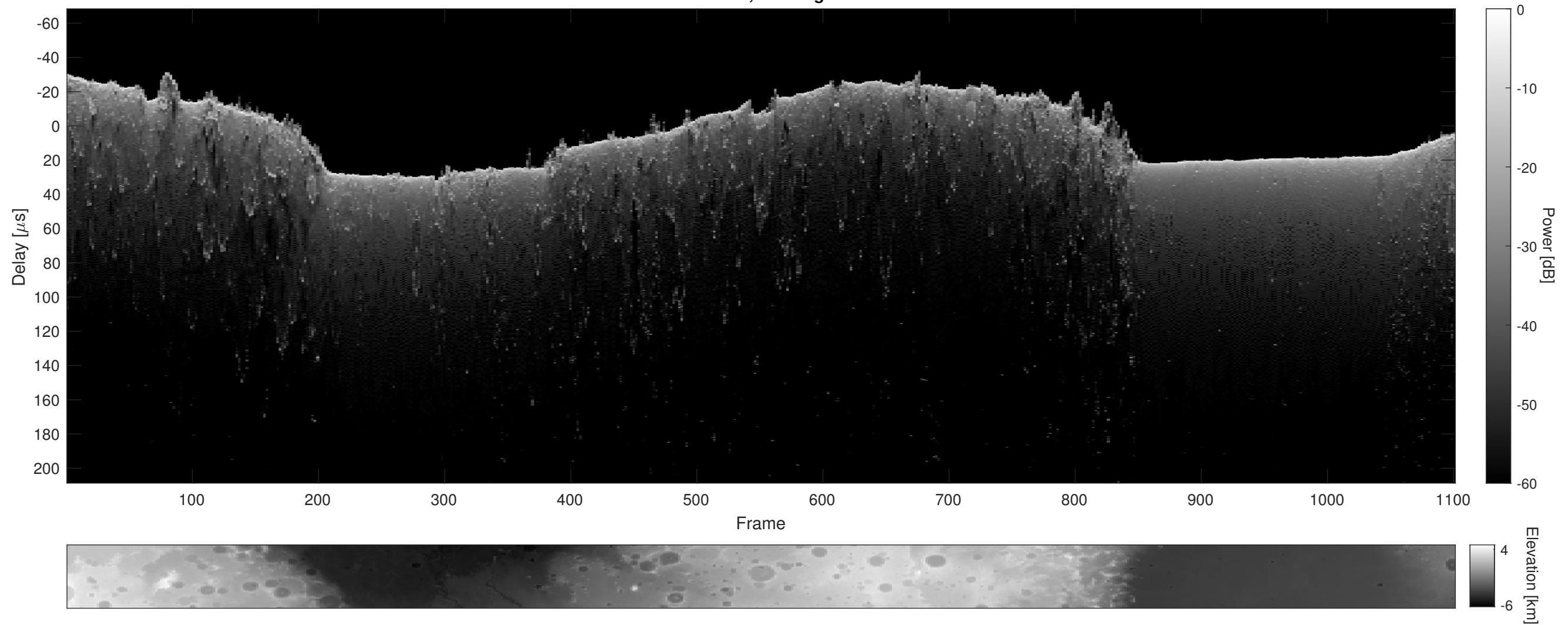
Orbit 2162, Cluttergram
