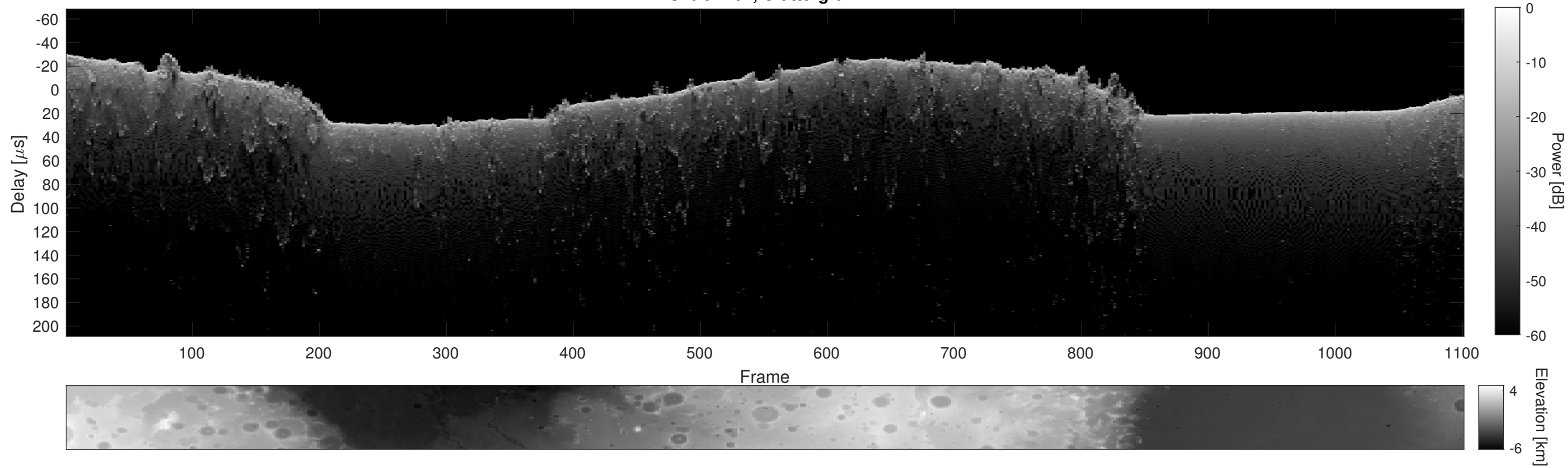
Orbit 2162, Cluttergram
