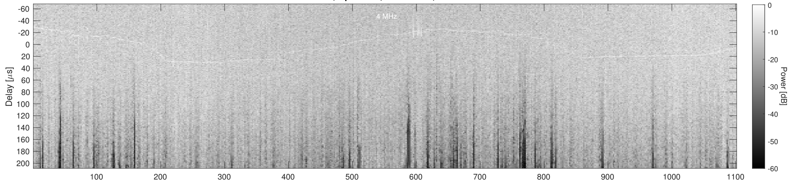
Orbit 2162, Cluttergram
