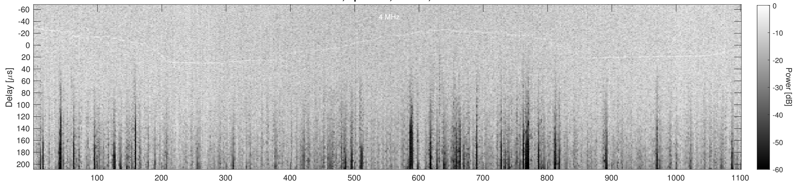
Orbit 2162, Cluttergram
