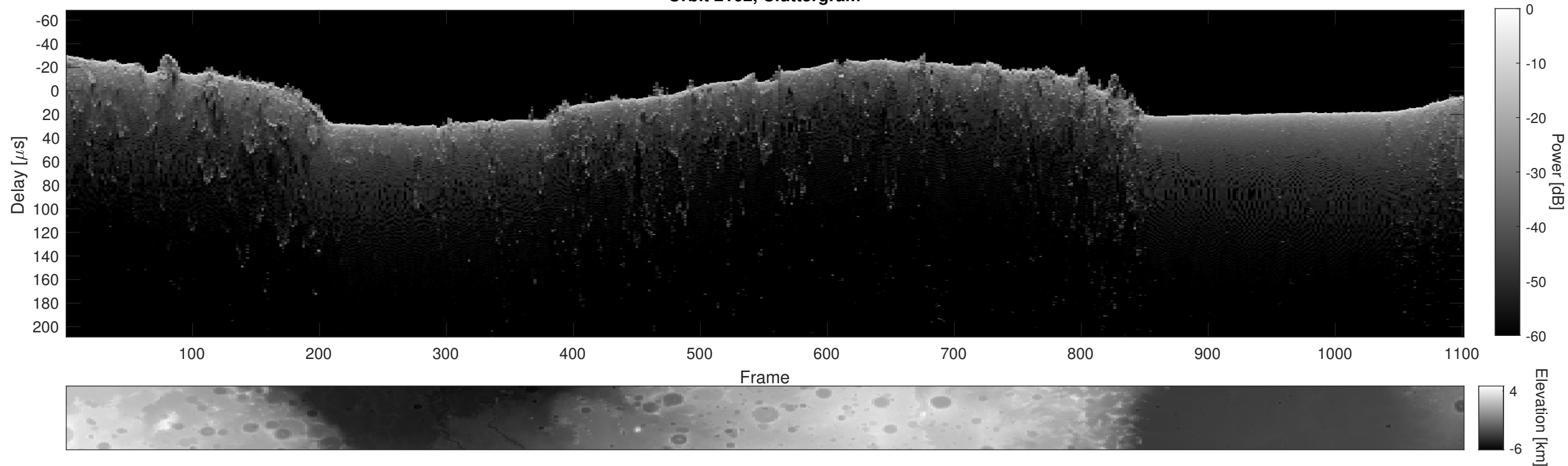
Orbit 2162, Cluttergram
