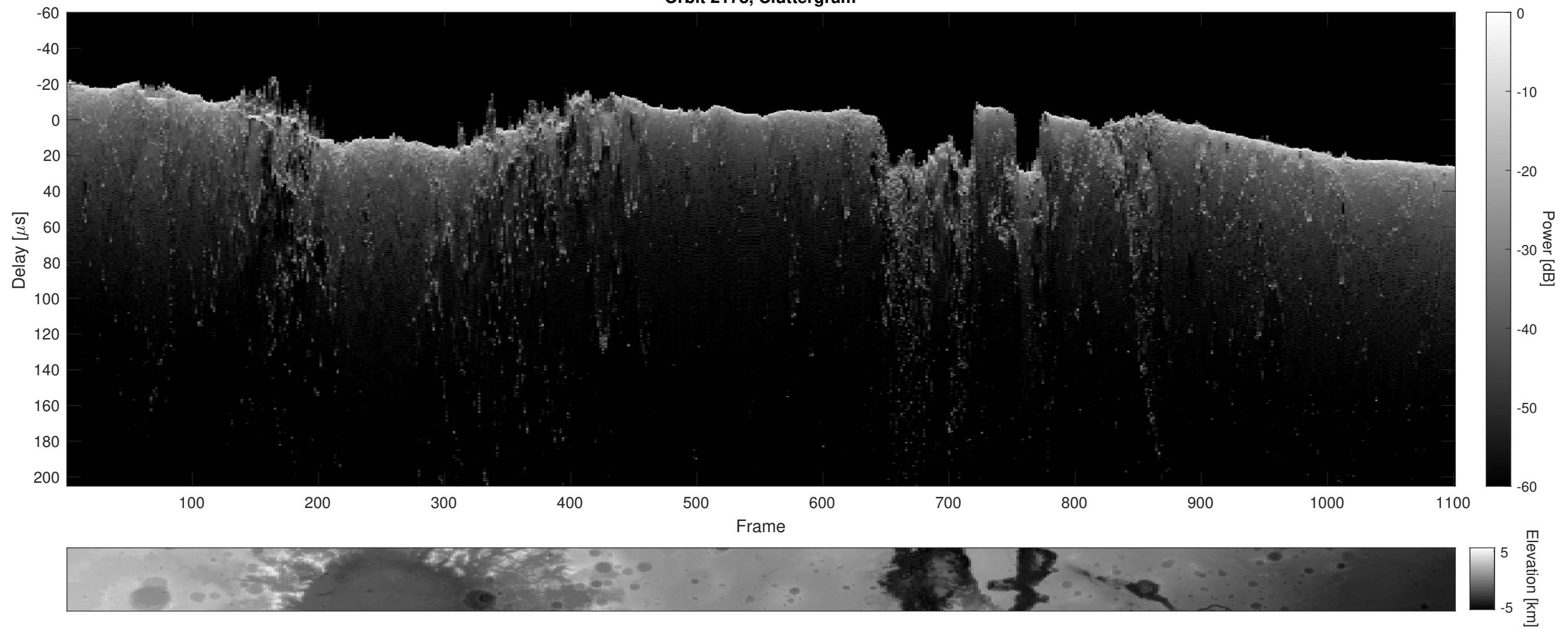
Orbit 2178, Cluttergram
